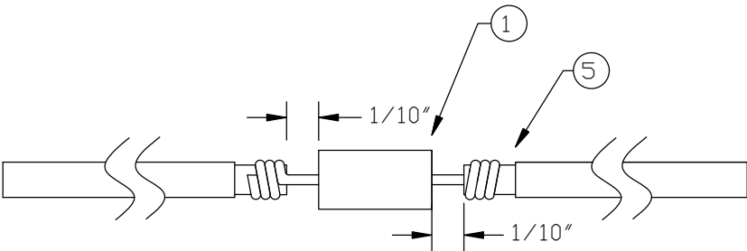
DETAIL D
