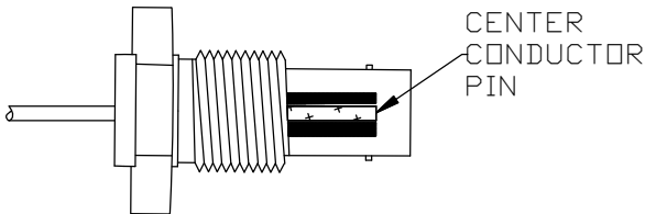
DETAIL B
