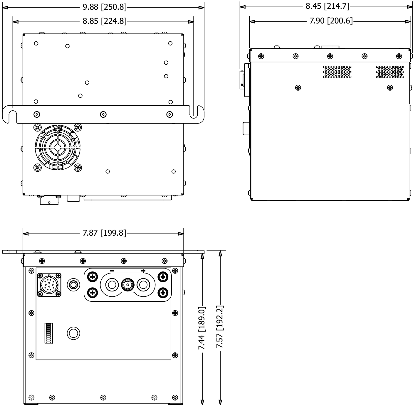
Figure 2.4.1 - TIUH60 MPU-24 physical dimensions
