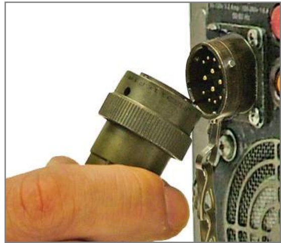
Figure 3.11.2 Attaching AC Line Cord
