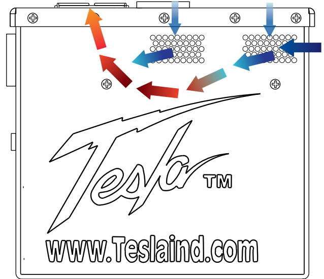
Figure 2.5.1 – Air intake and exhaust ports and internal air circulation
