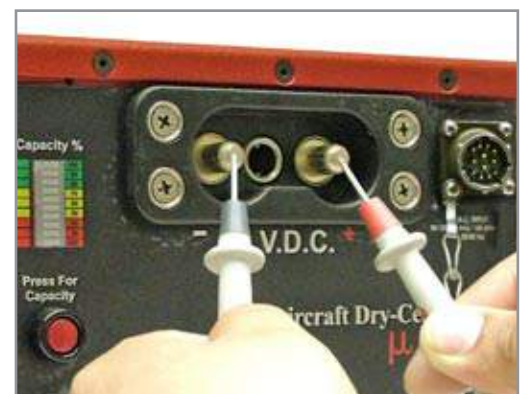
Figure 3.8.3 – Testing DC Receptacle
