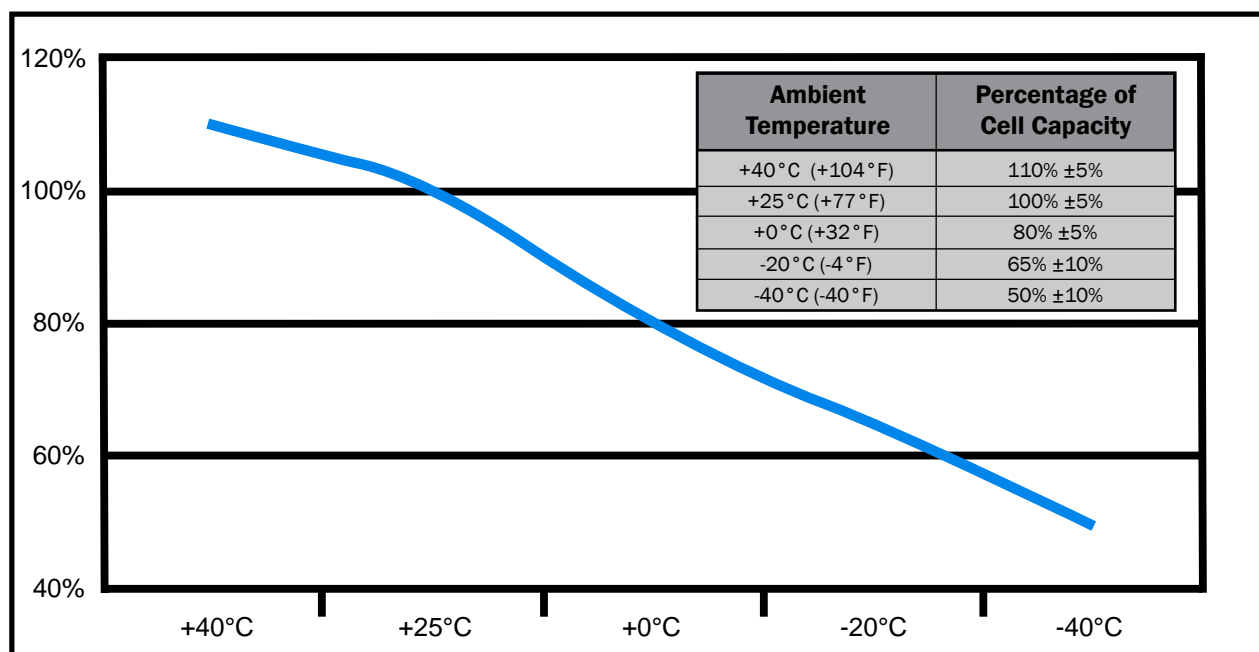
Figure 3.6.1 – Cell storage capacity versus ambient temperature
