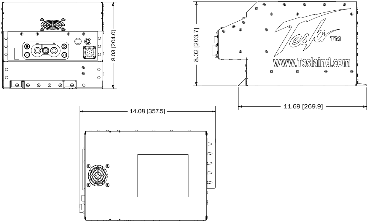
Figure 2.5.1– TI47407 MPU-24 physical dimensions
