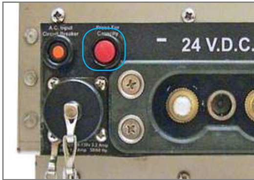
Figure 2.8.1 “Press for Capacity” button location (outlined in blue)
