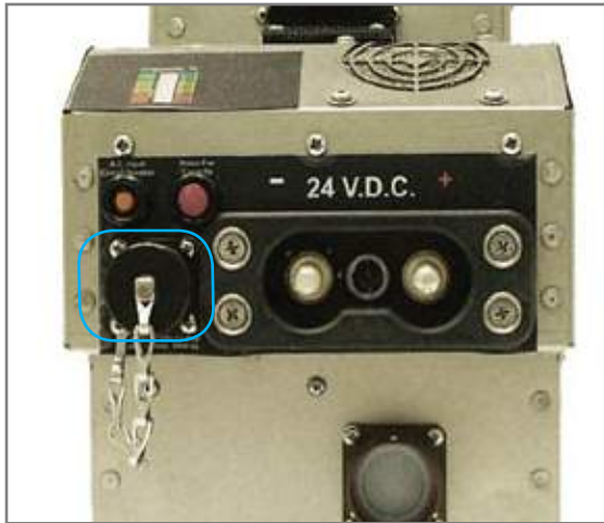
Figure 3.12.1 AC Input Connector (outlined in blue)
