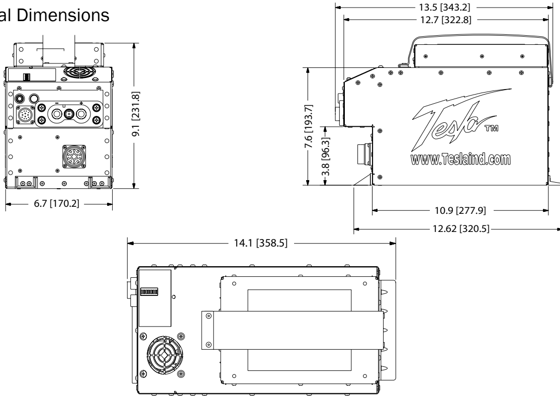
Figure 2.5.1 – TI58D MPU-24 physical dimensions
