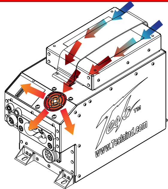
Figure 2.6.1 – Air intake and exhaust ports and internal air circulation
