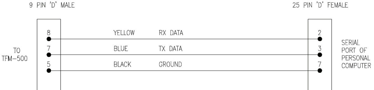
FIGURE 2.2 TFM-530 Transceiver PC Up/Download Cable - wiring diagram
