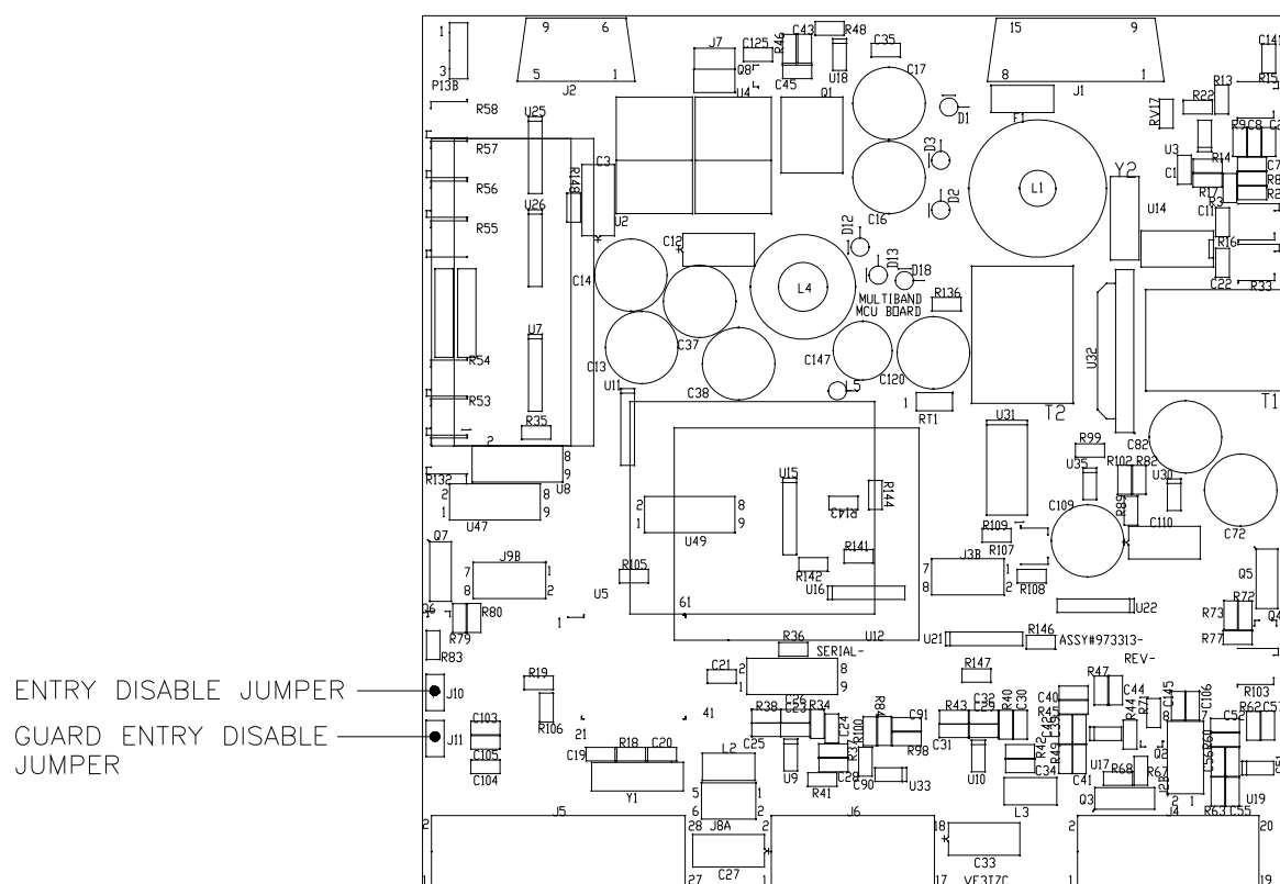
FIGURE 3.4 Internal Enable/Disable Jumper Locations
