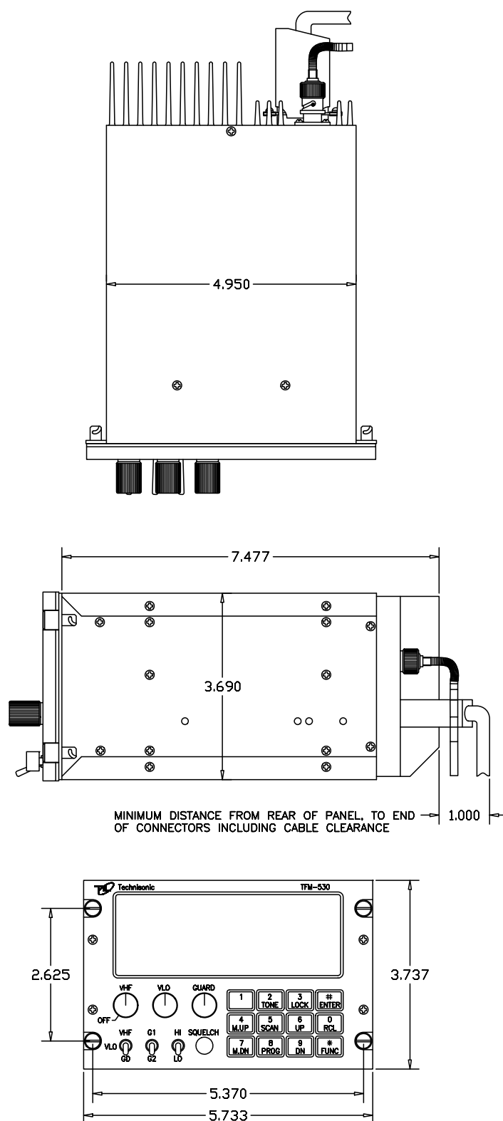
FIGURE 3.1 Outline Drawing for Model TFM-530 Series Transceivers
