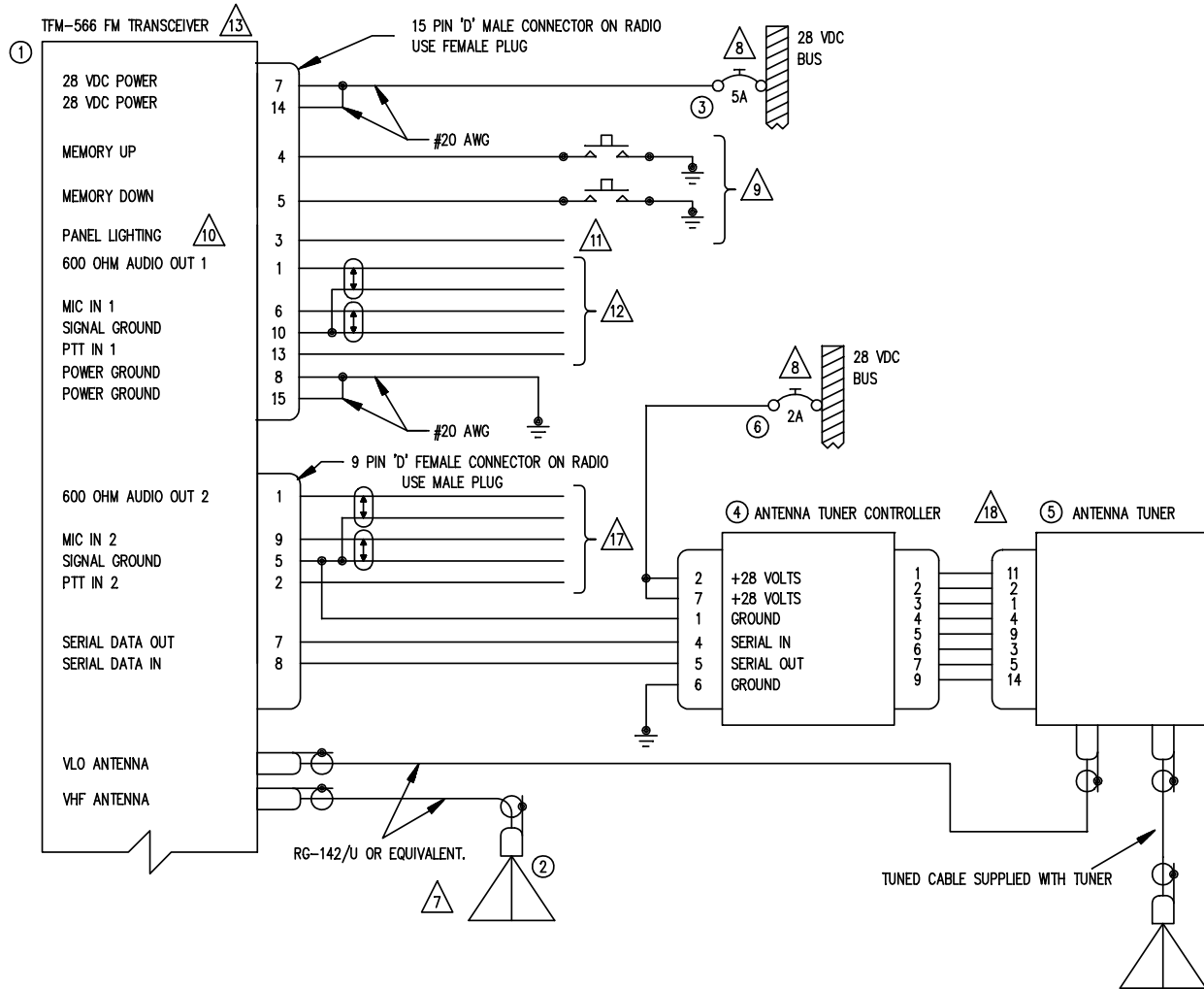
FIGURE 3.2 Wiring connections for the TFM-566 Transceiver
