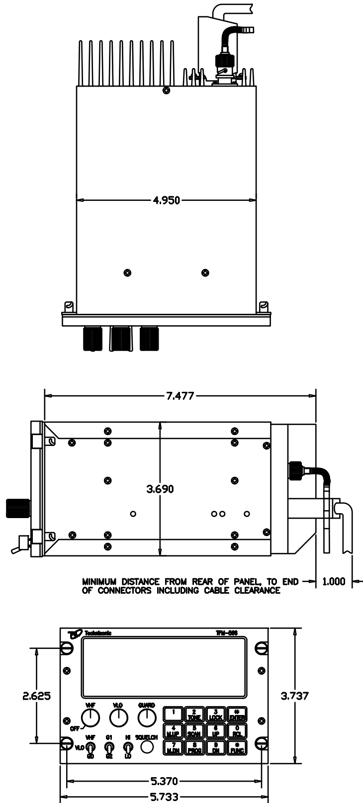
FIGURE 3.1 Outline Drawing for Model TFM-566 Series Transceivers
