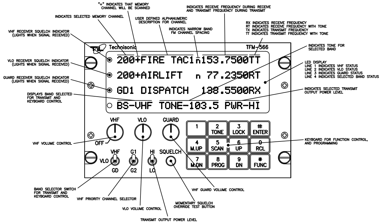
FIGURE 2.1 Operator's Switches and Controls
