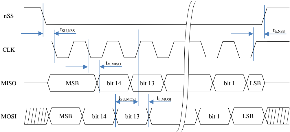
Figure 17 SPI Timing Diagram
