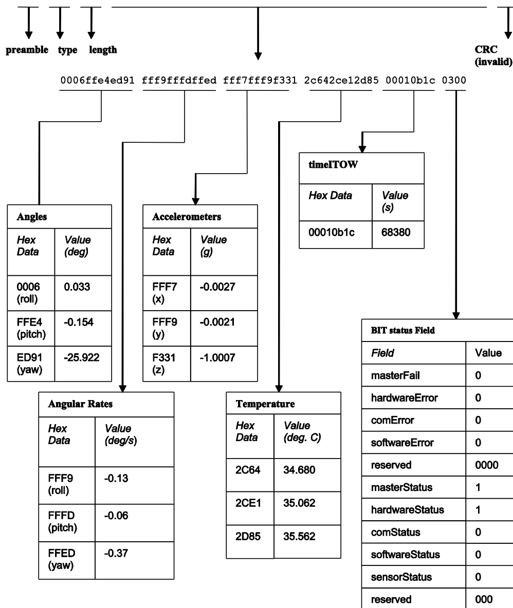
Figure 30 Example payload from Angle Data Packet 2 (A2)
