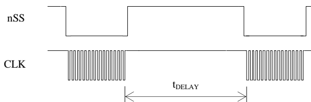
Figure 16 Delay Time
