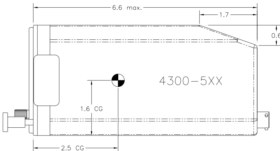
Figure 2.1 Outline Drawing
