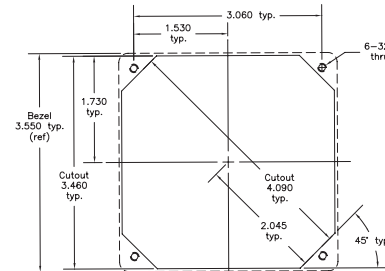
4300 Series Front-Mount Panel Cutout
