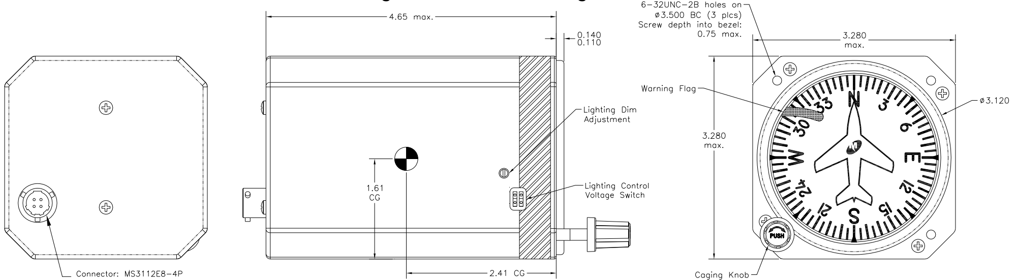
Figure 2.1 Outline Drawing
